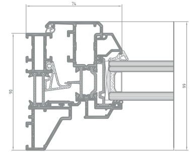
STEEL LOOK 1000 window section
